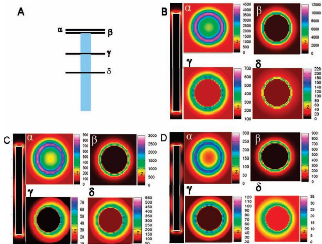
Figure 2. (A) Scheme of the planes \alpha , \beta , \gamma , and \delta perpendicular to the Ag NW axis ( L = 480 nm, D = 40 nm), where the |E|^2 distributions are shown. Cross-sectional distributions of |E|^2 on planes \alpha , \beta , \gamma , and \delta for the (B) dipole, (C) quadrupole, and (D) octupole mode.
